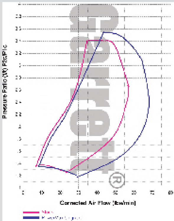
Compressor Map
