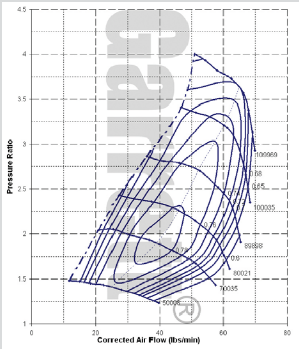
Compressor Map
