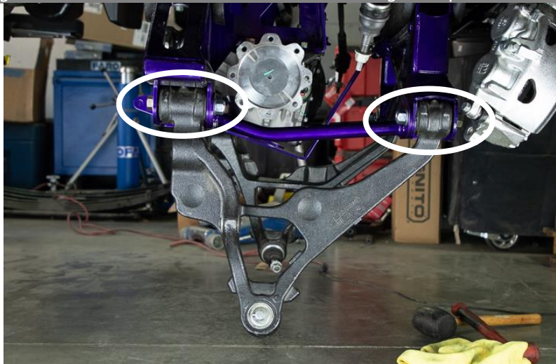
Figure 72: Lower Control Arm Bolts that do NOT get torqued at this step
